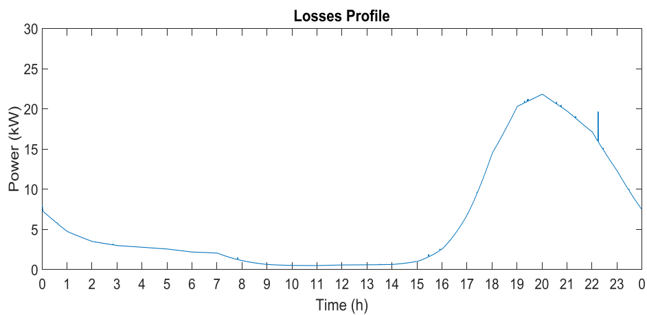
Figure 15. Generator profile.
