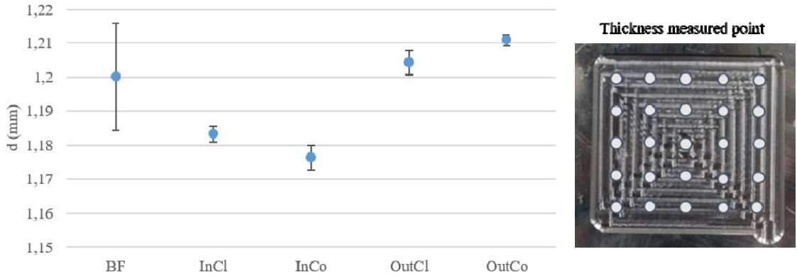
Fig. 6. Thickness average results depending on the toolpath.
