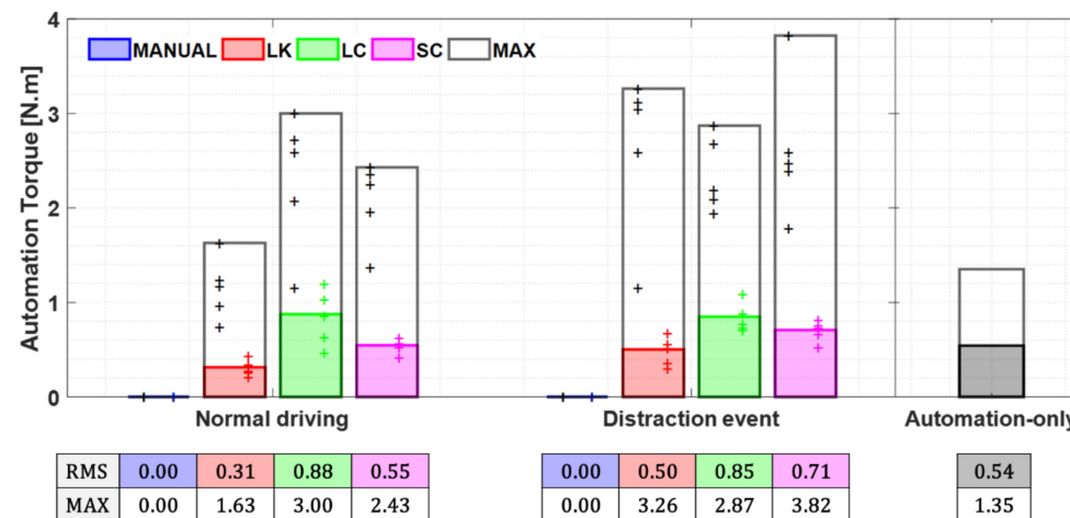
Figure 14. Driving efforts statistics (RMS and MAX of automation’s torque).
