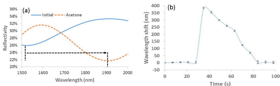
Fig. 11. (a) FTIR measured spectra for the PA6 NFs FP sensing layer being filled with air (initial spectrum) and when acetone is deposited over the sample. (b) Temporal evolution of the spectral shift measured for the PA6 NFs FP sensing layer (error bars included).
